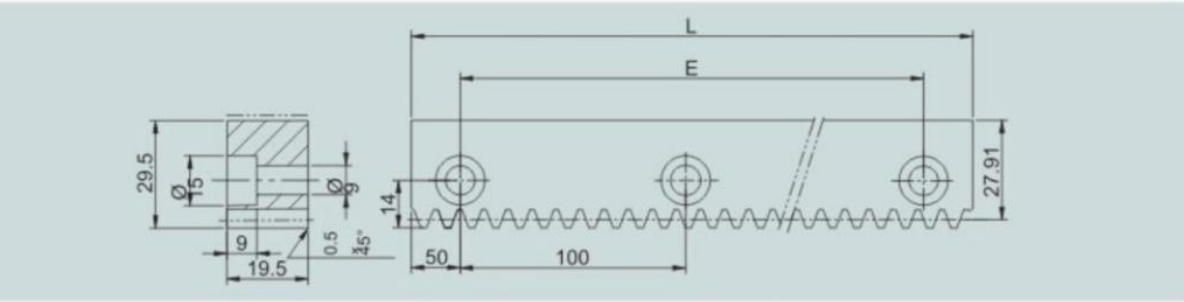
导轨齿条 Guideway fat rail rack
