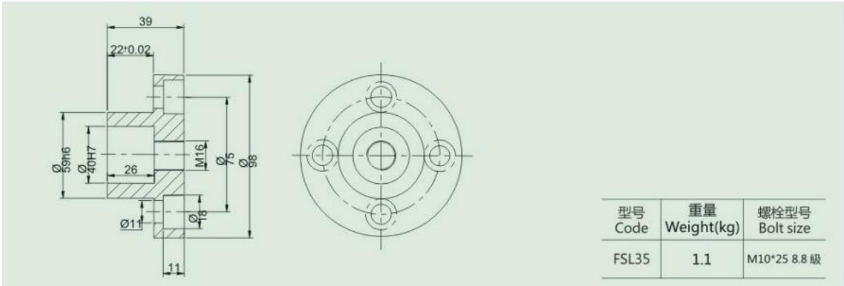
Mounting fange
