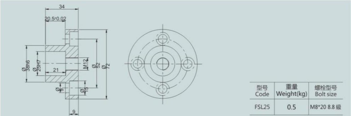
Mounting fange
