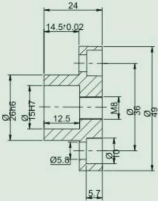
Mounting fange
