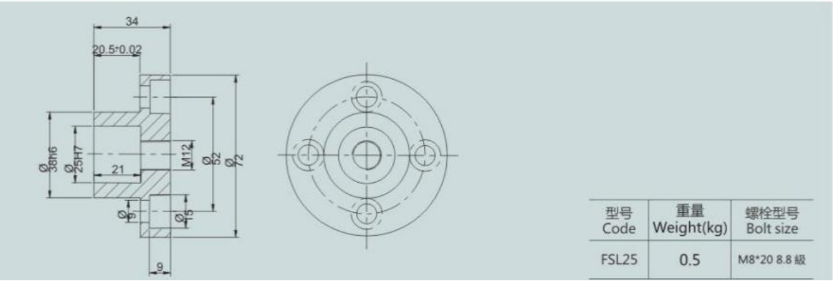
Mounting fange
