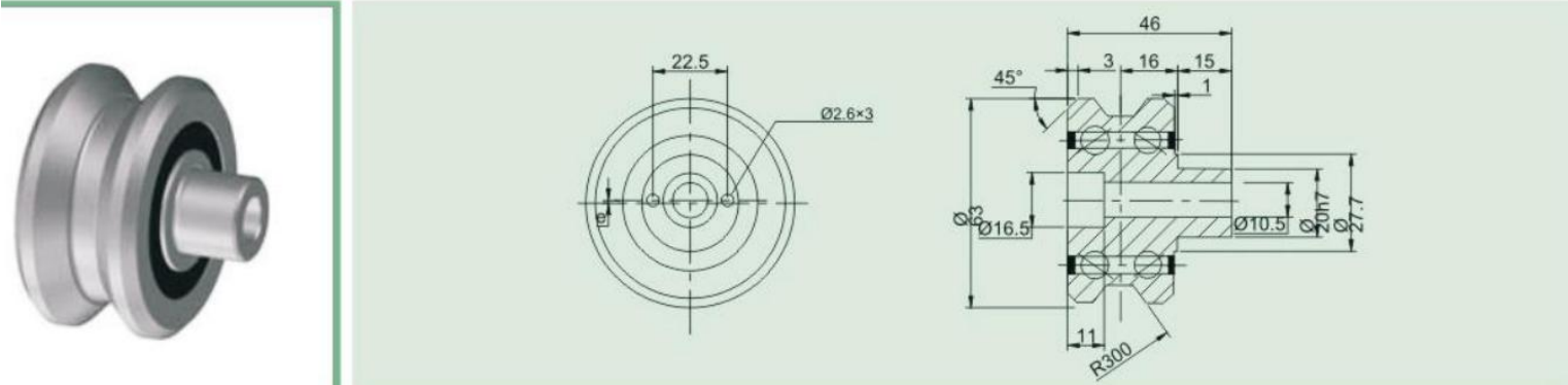
滚轮Roller for guideway V bars
