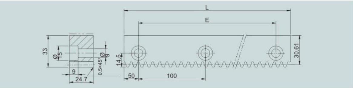
导轨齿条 Guideway fat rail rack
