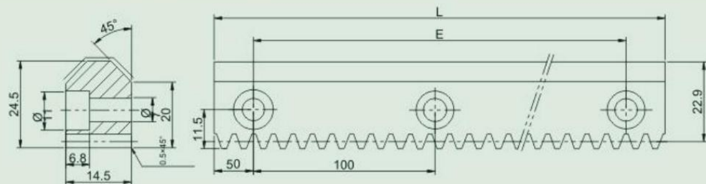
导轨齿条 Guideway V bar rack
